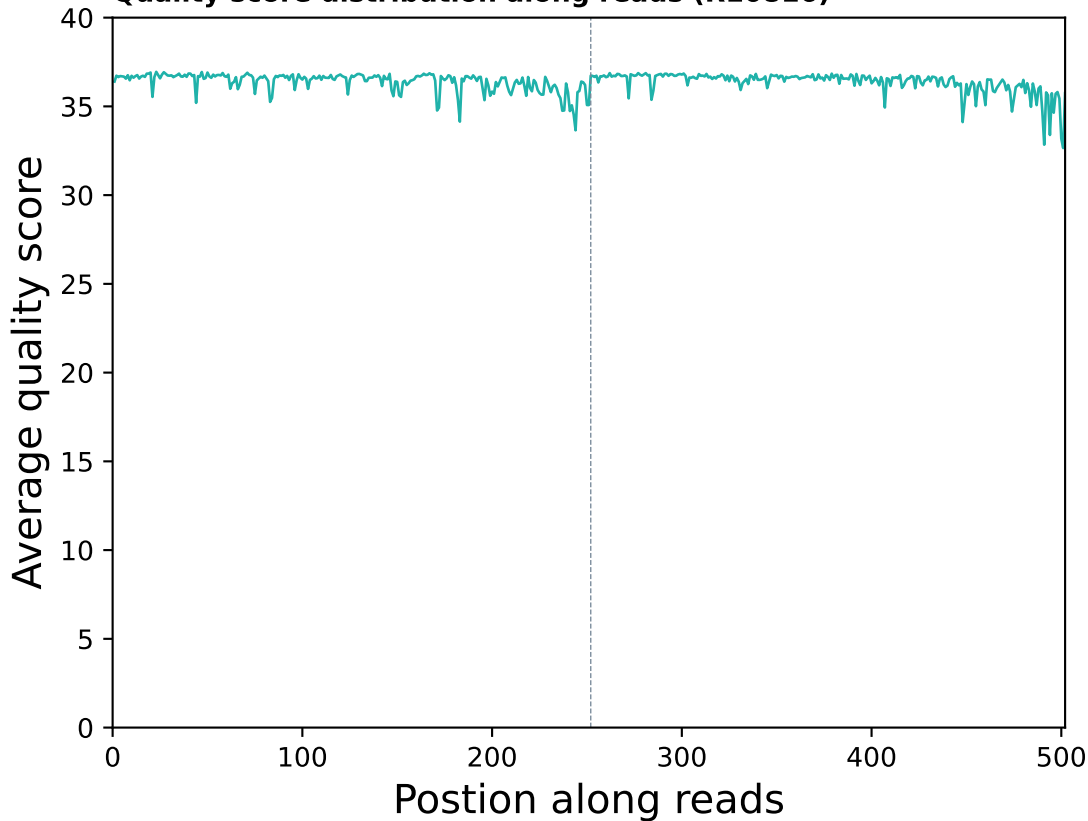
Quality score distribution along reads (R10816)
